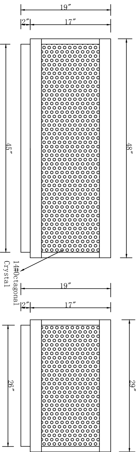
Front view
